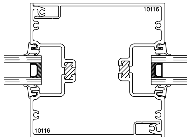
13 4" MULLION
