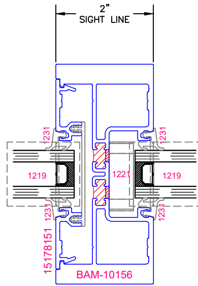
11 HEAVY DUTY MULLION
