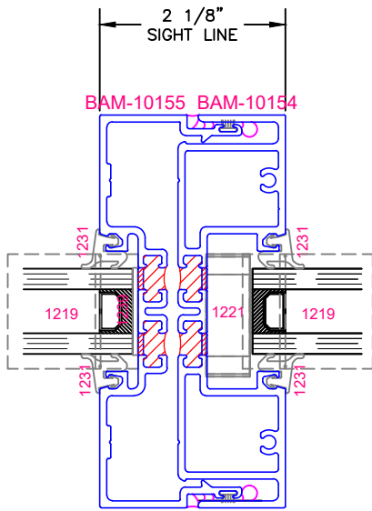
10 EXPANSION MULLION
